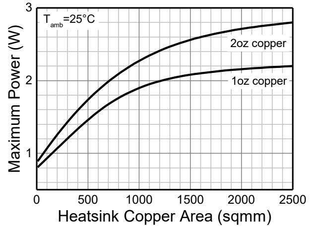
Fig.2 Max Power Dissipation vs. Copper Area
