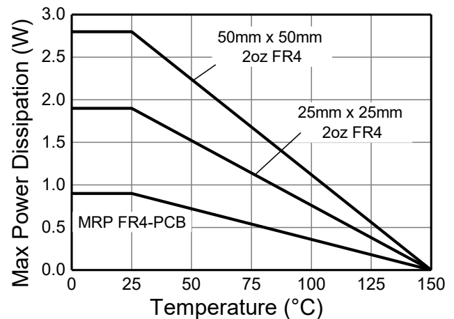
Fig.6 Derating Curve
