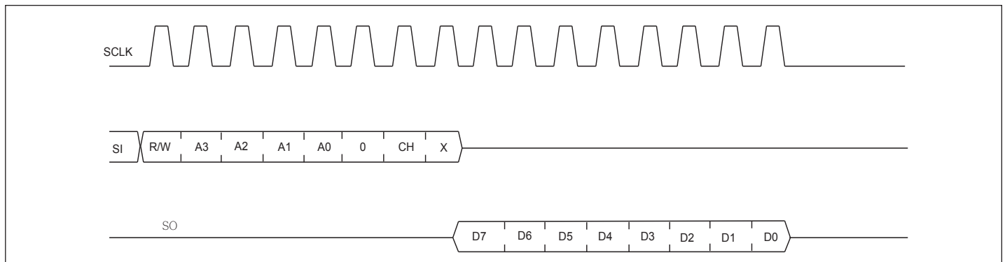
Figure 14. SPI Read
