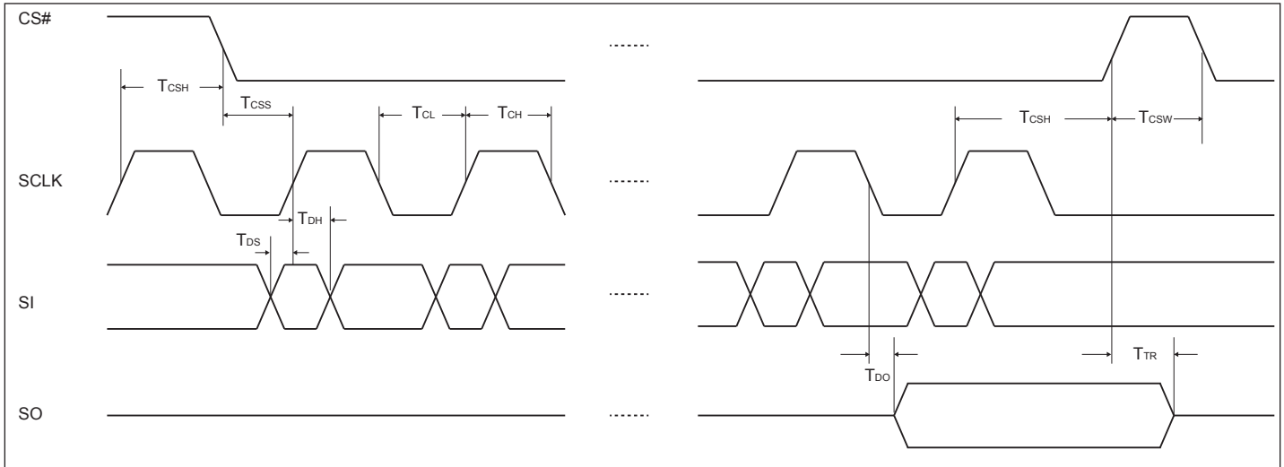
Figure 26. SPI-Bus Timing
