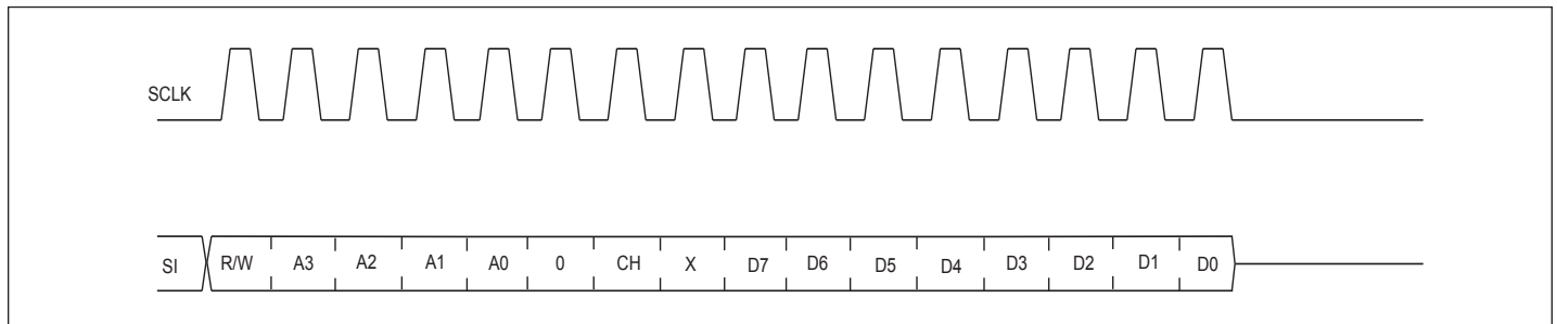
Figure 13. SPI Write
