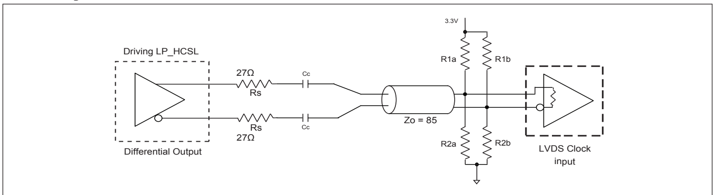
Figure 3. Differential Output Driving LVDS
