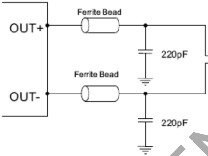
Figure 2. Ferrite Bead Filter to Reduce EMI
