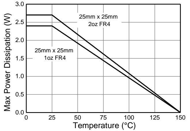
Figure 2. Derating Curve
