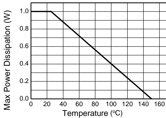
Figure 2. Derating Curve
