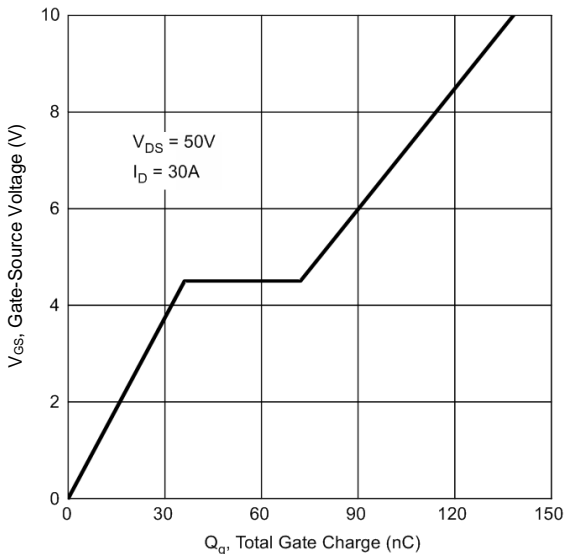
Fig. 11 Gate Charge
