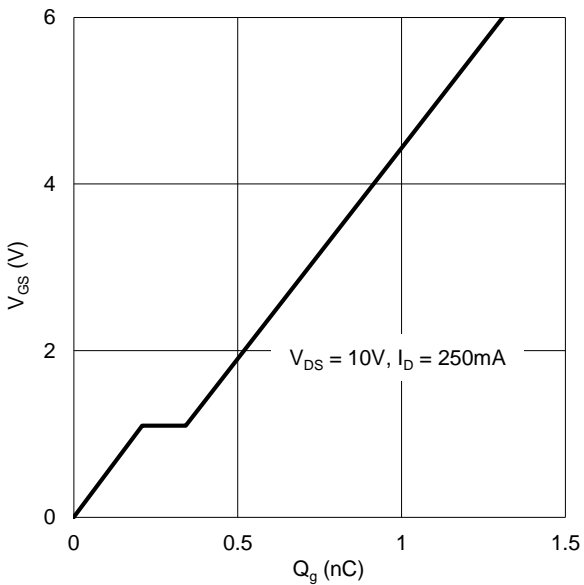
Figure 11. Gate Charge
