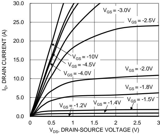
Figure 14. Typical Output Characteristic
