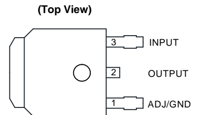
TO252-2 (4)
