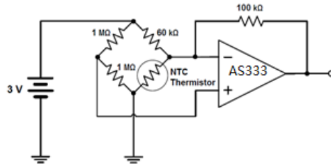
Figure 8. Bridge Circuit Amplification
