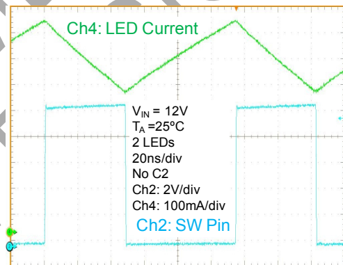
Figure 32 Typical Operating Waveform (C2 not fitted)
