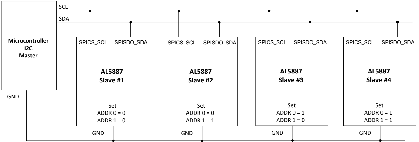
3) Four AL5887 connected together with external hardware pins setup
