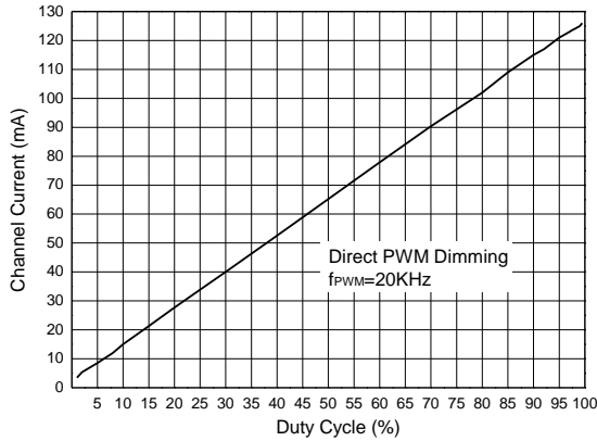
Direct PWM Dimming @ f_{\text{PWM}} = 20\text{kHz} Channel Current vs. Duty Cycle
