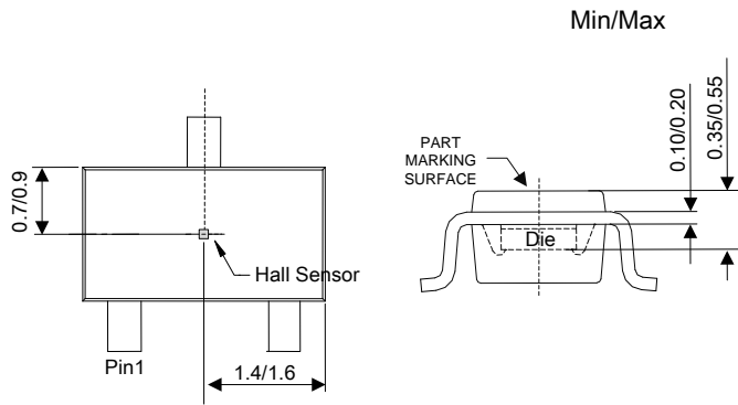
Sensor Location
