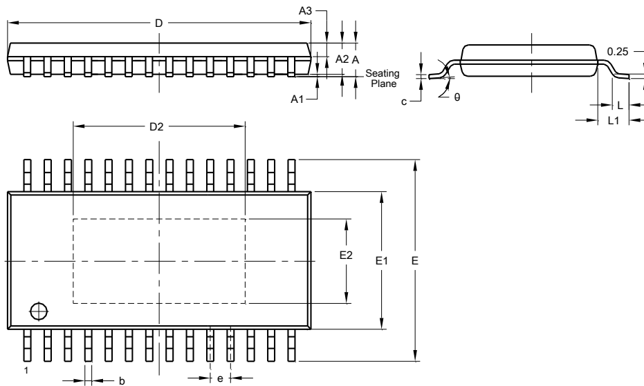
TSSOP-28EP (Type TH-1)
