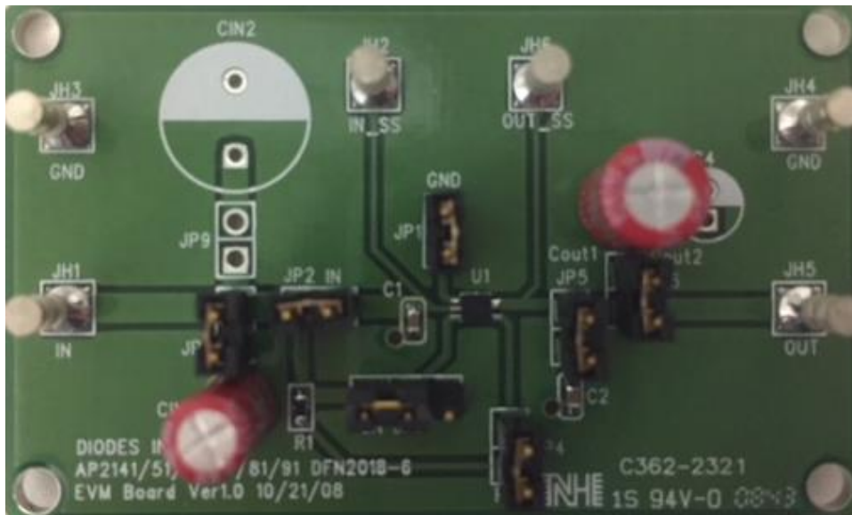
Figure 1 . AP21X10FMG-EVM
