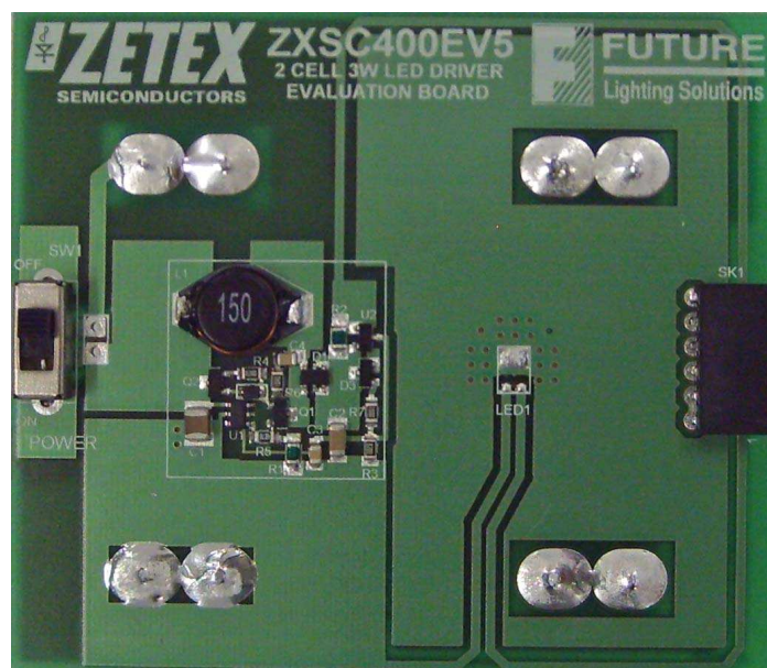
Figure 1. ZXSC400EV5 Evaluation Board.
