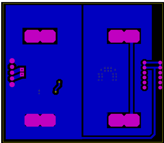
Bottom Copper
