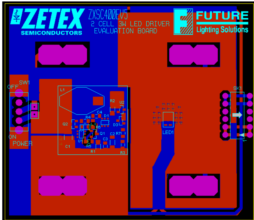
Figure 4. Evaluation PCB
