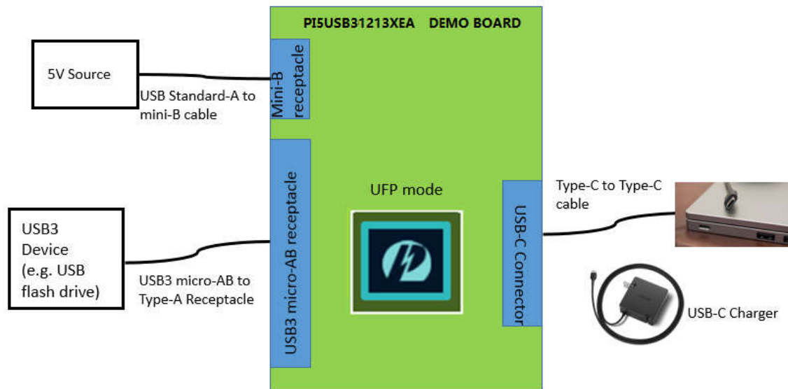
Figure 4: PI5USB31213 Demo Board battery-powered UFP mode illustration.
