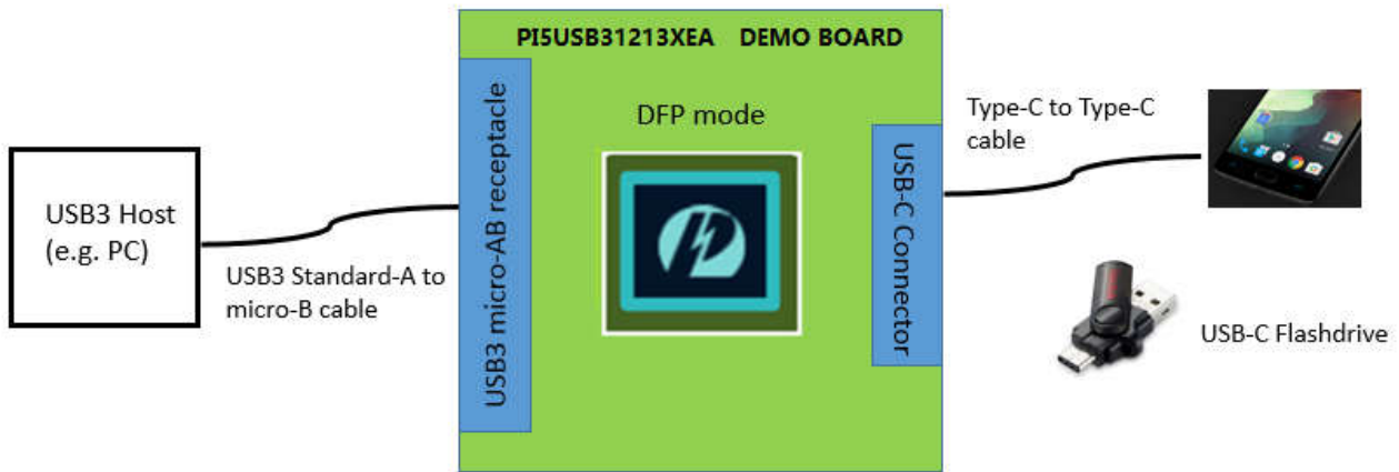
Figure 3: PI5USB31213 Demo Board DFP mode illustration.
