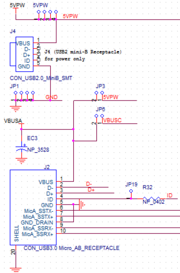
Figure 7: Power Supply option of PI5USB31213 Demo Board Rev.B
