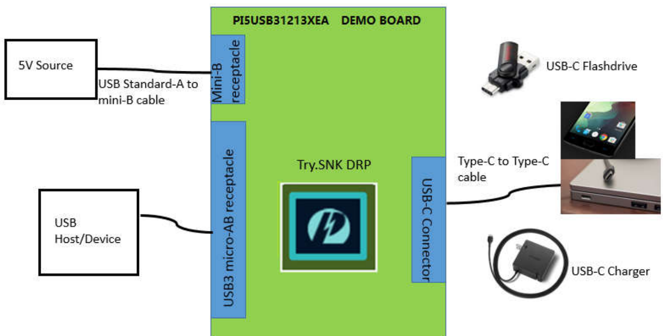
Figure 5: PI5USB31213 Demo Board Try.SNK DRP mode illustration.
