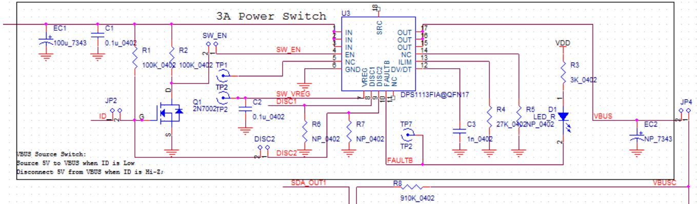
Figure 6: VBUS switch of PI5USB31213 Demo Board Rev.B
