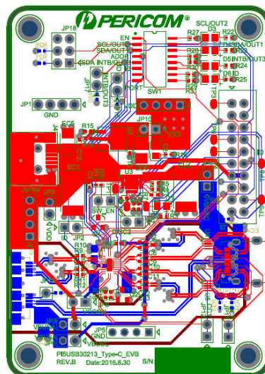
Figure 2: Layout of PI5USB31213 Demo Board Rev.B
