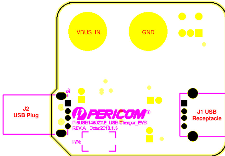
Figure 5, Bottom view of PI5USB1458/PI5USB1458A EVB Layout
