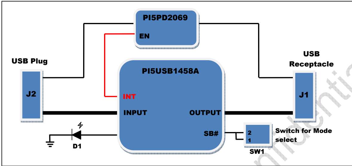
Figure 1b, block diagram of PI5USB1458A EVB
