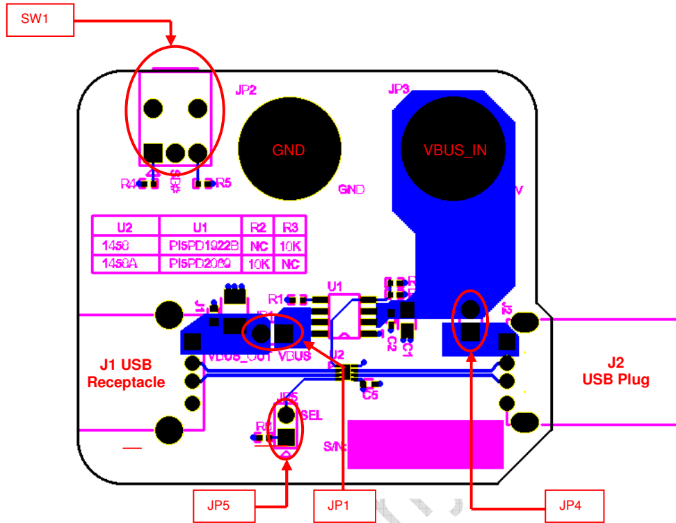
Figure 4, Top view of PI5USB1458/PI5USB1458A EVB Layout
