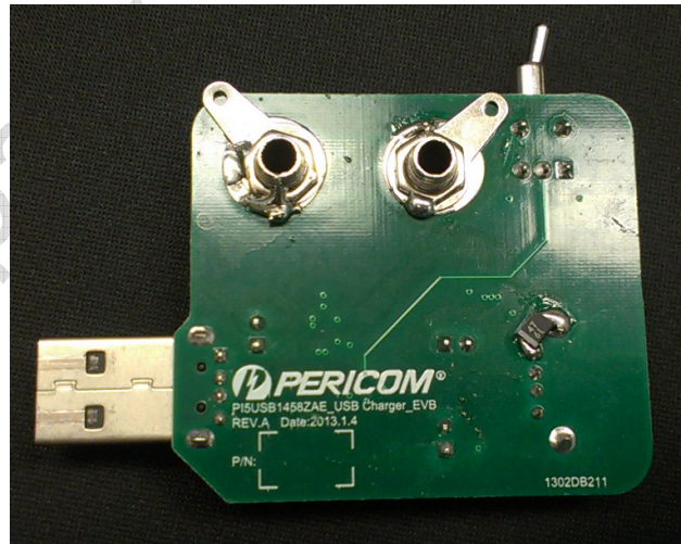
Figure 2(b), bottom view of PI5USB1458/PI5USB1458A EVB
