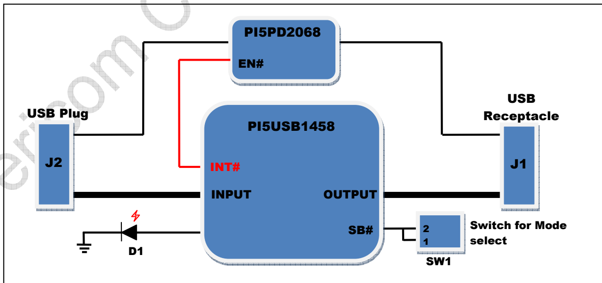
Figure 1a, block diagram of PI5USB1458 EVB
