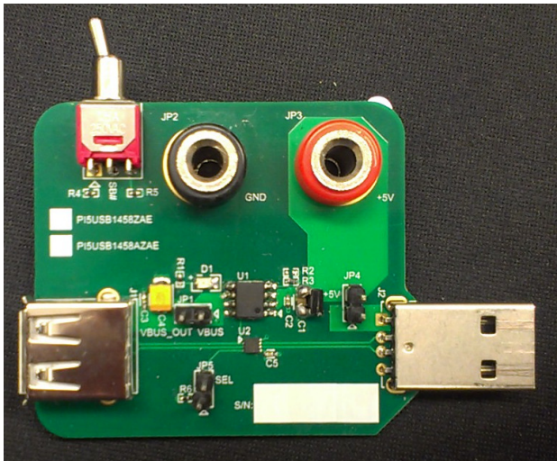
Figure 2(a), top view of PI5USB1458/PI5USB1458A EVB
