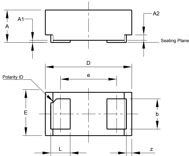
X4-WLB0402-2 (SWP)
