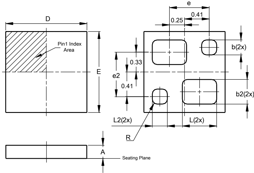
X4-DSN1313-4
