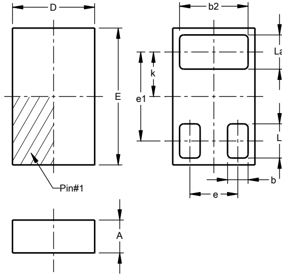
X4-DSN1006-3
