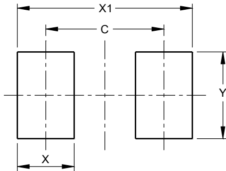
X4-DSN0603-2
