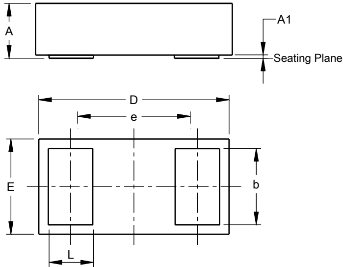
X4-DSN0603-2
