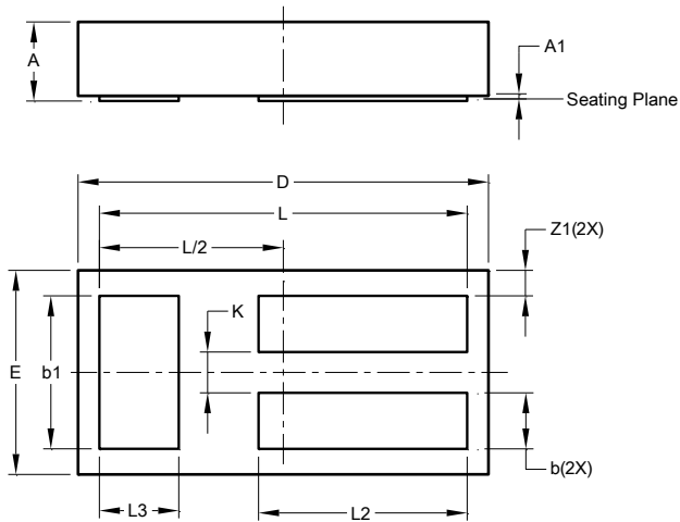
X2-WLB1608-3
