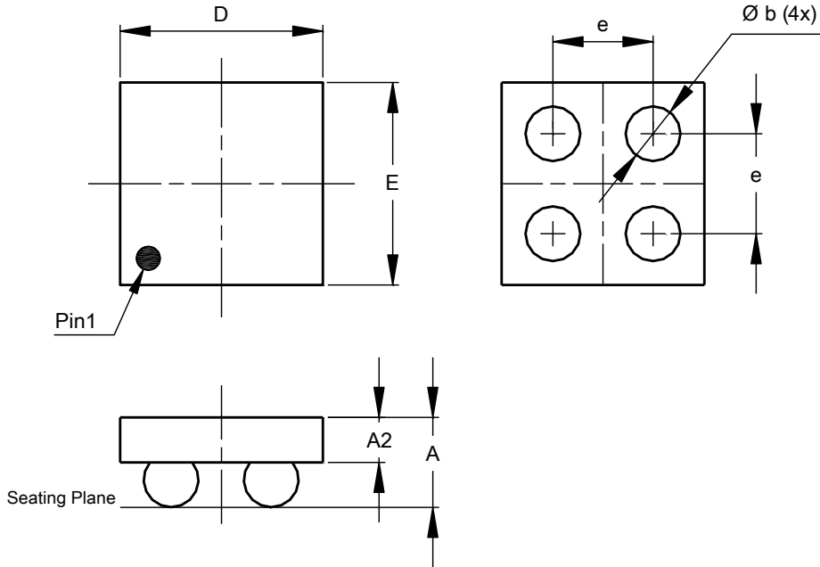
X2-WLB0808-4
