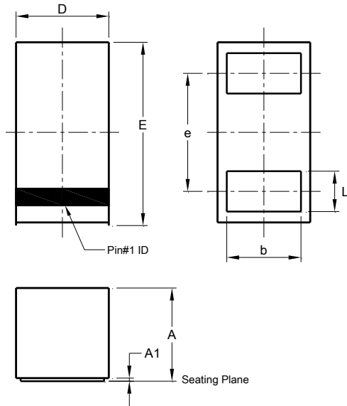
X2-WLB0603-2
