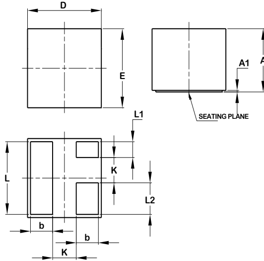
X2-WLB0505-3
