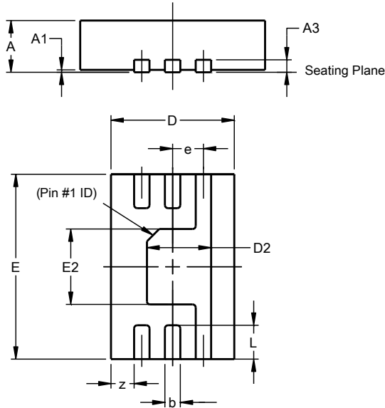
X2-DFN3020-6
