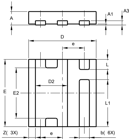
X2-DFN2020-6
