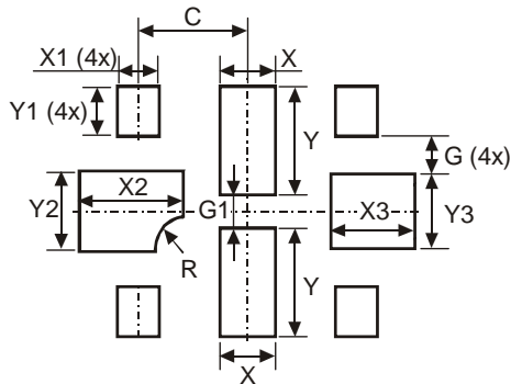
X2-DFN2015-8
