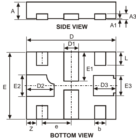
X2-DFN2015-8
