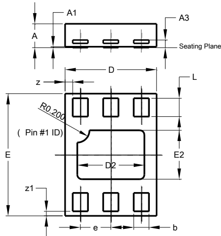
X2-DFN2015-6
