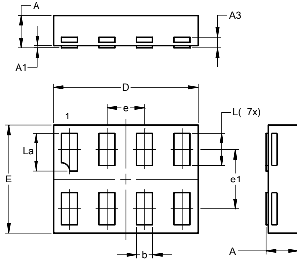
X2-DFN1410-8
