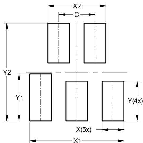
X2-DFN1410-5 (Type A)
