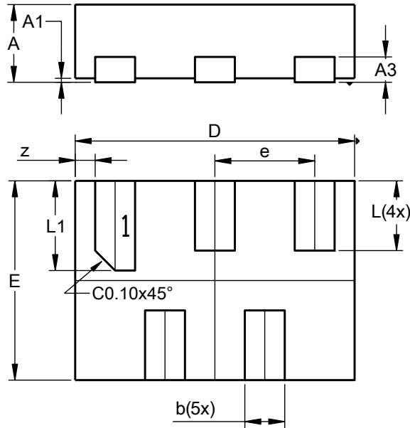
X2-DFN1410-5 (Type A)
