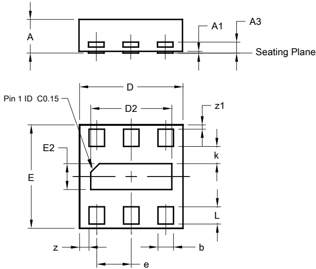
X2-DFN1212-6
