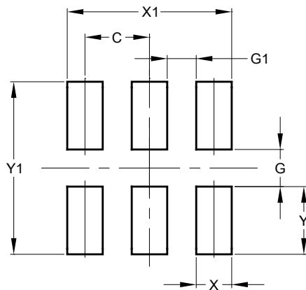
X2-DFN1210-6
