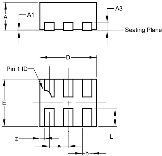
X2-DFN1210-6
