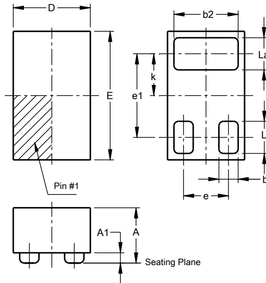
X1-DSN1006-3
