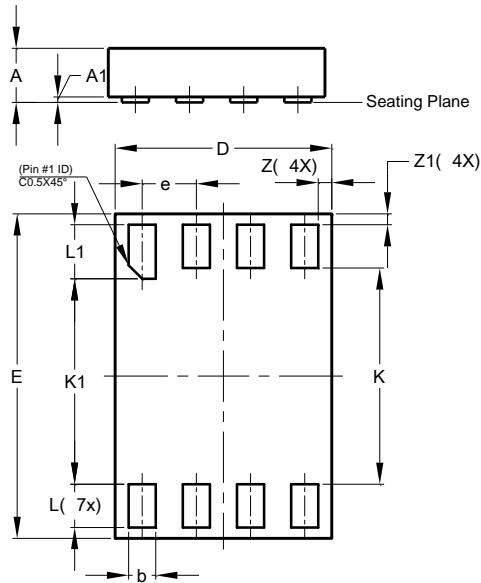
X1-DFN2030-8
