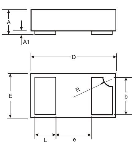
X1-DFN1006-2
