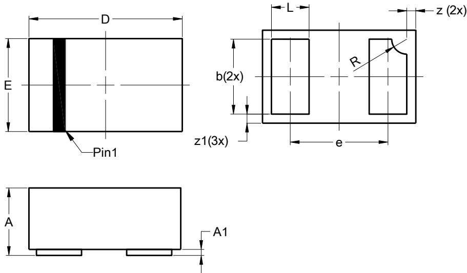
X1-DFN1006-2 (Type SA)
