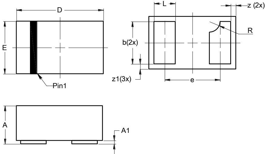
X1-DFN1006-2 (Type SA-2)
