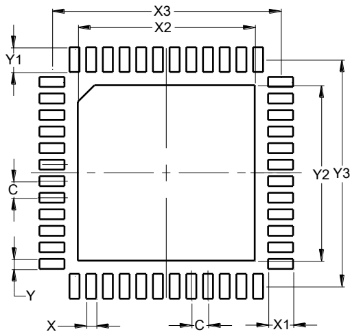
W-QFN7070-48/SWP (Type A1)
