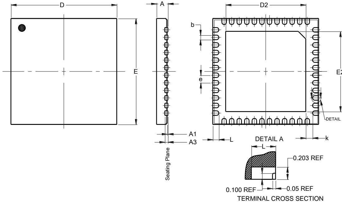
W-QFN7070-48/SWP (Type A1)
