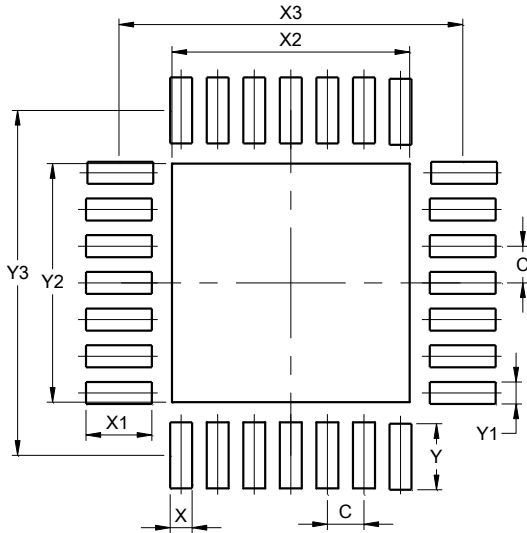
W-QFN5050-28 (Type A1)
