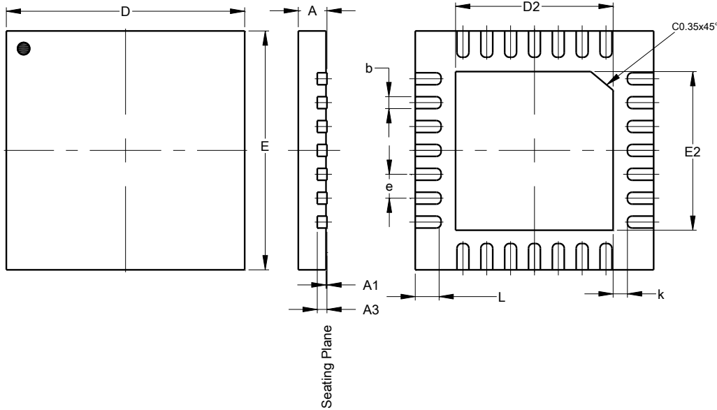
W-QFN5050-28 (Type A1)
