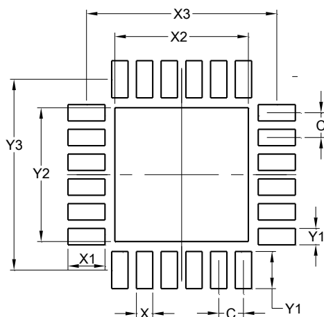
W-QFN4040-24/SWP (Type A1-B)
