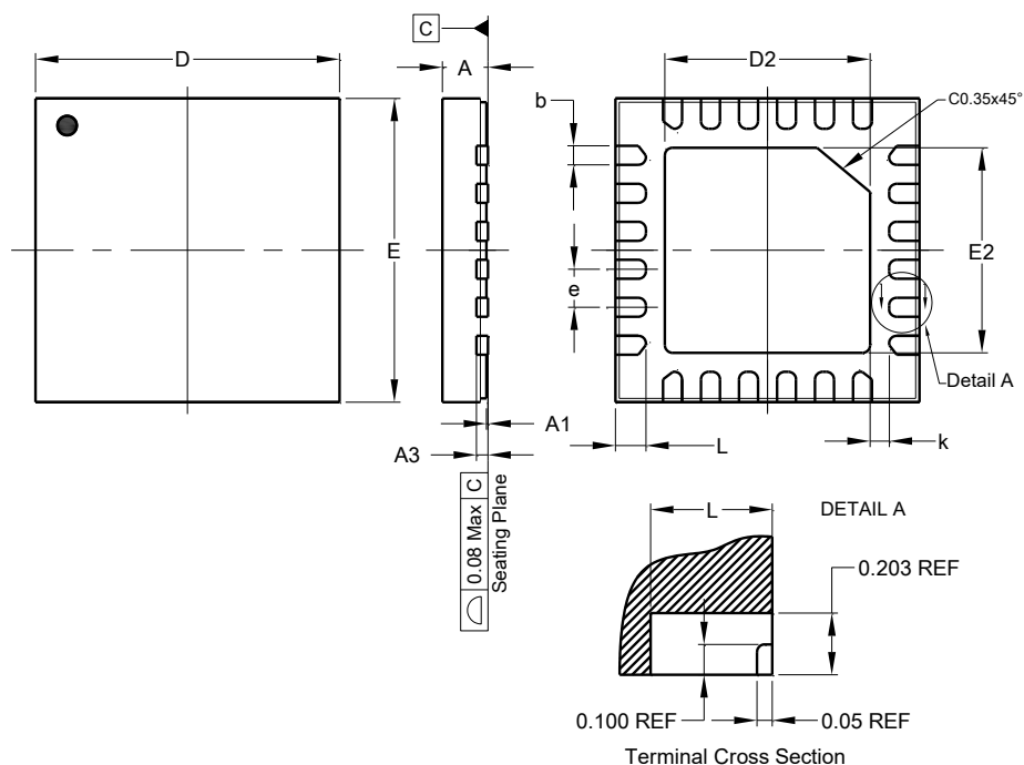
W-QFN4040-24/SWP (Type A1-B)
