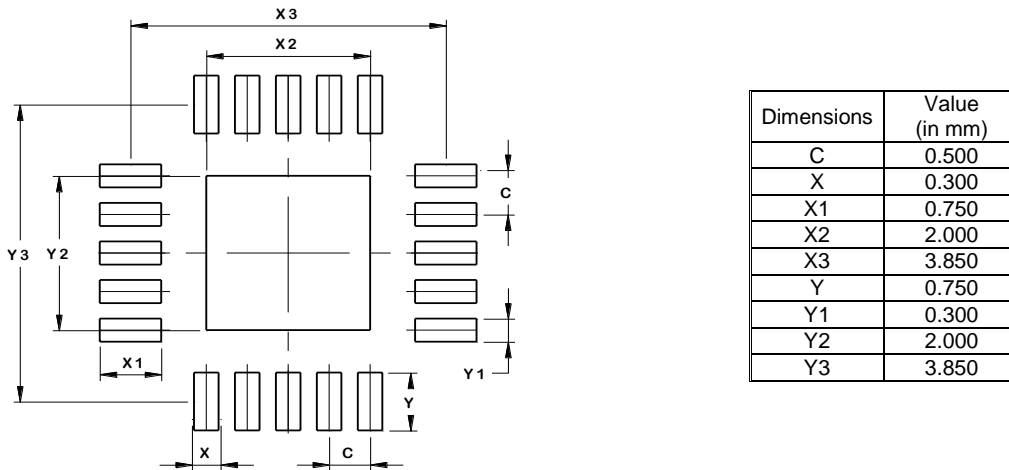
W-QFN4040-20 (SWP) (Type A1)
