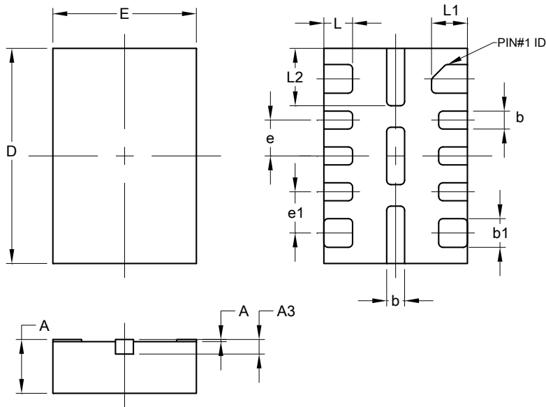
W-QFN3020-12
