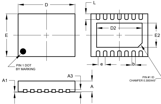
W-DFN4030-14
