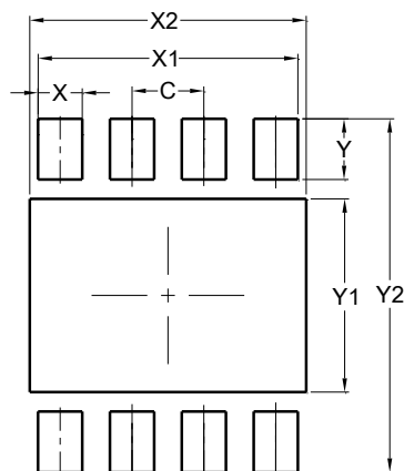
W-DFN3030-8 (Type UXF)
