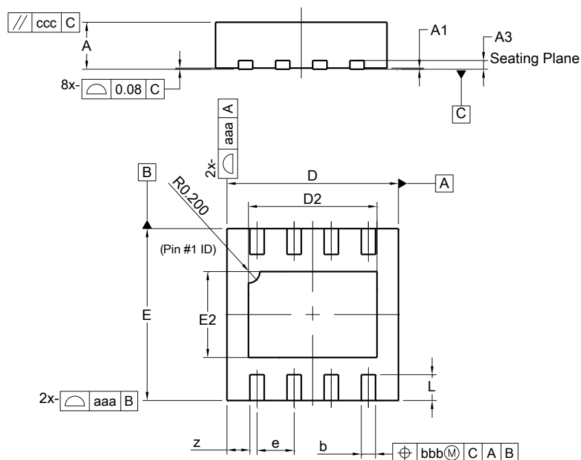
W-DFN3030-8 (Type UXF)
