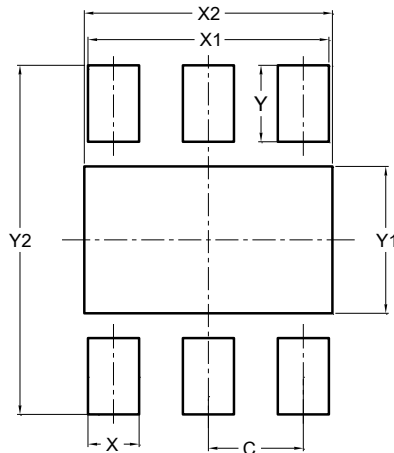
W-DFN2020-6 (SWP) (Type UXD)
