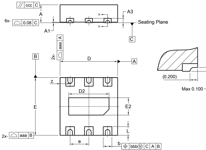
W-DFN2020-6 (SWP) (Type UXD)
