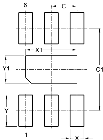
W-DFN2020-6 (SWP) (Type A1)
