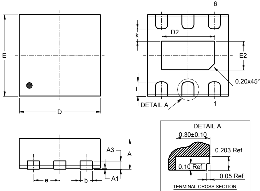
W-DFN2020-6 (SWP) (Type A1)
